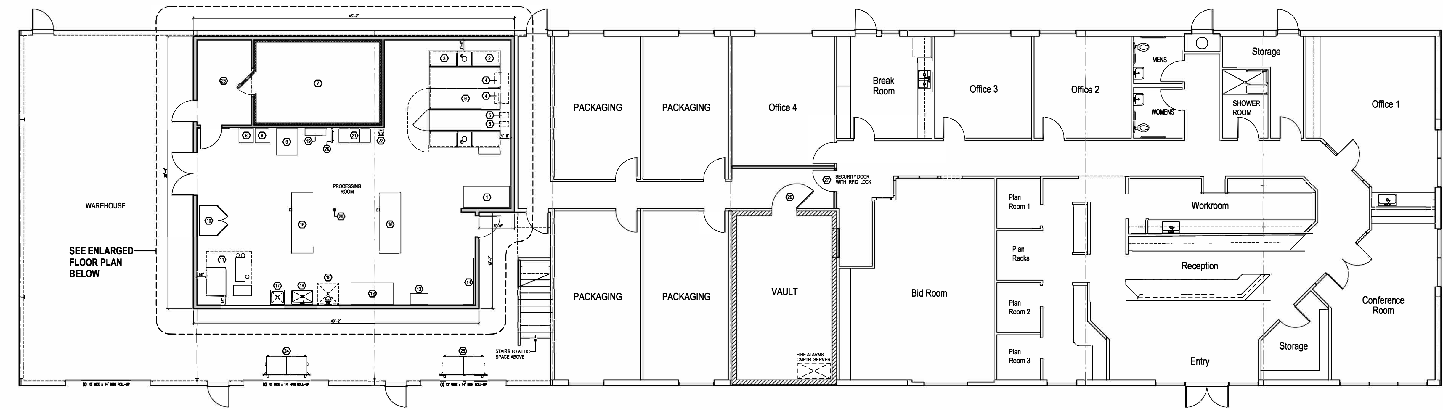
OVERALL FLOOR PLAN SCALE: 1/8" = 1'-0" EXISTING BUILDING: 10,000 S.F. NEW PROCESSING ROOM: 1664 S.F.
