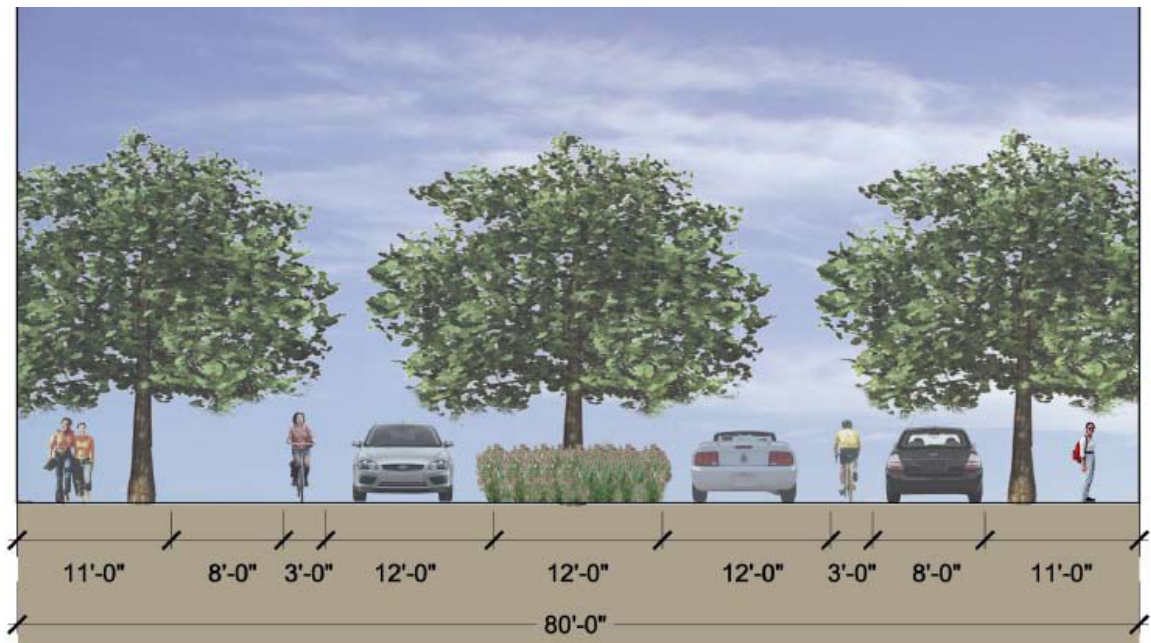
LOCAL COLLECTOR A+B - CAMPUS CORE EDGE ACCESS + CAMPUS CORE ACCESS
