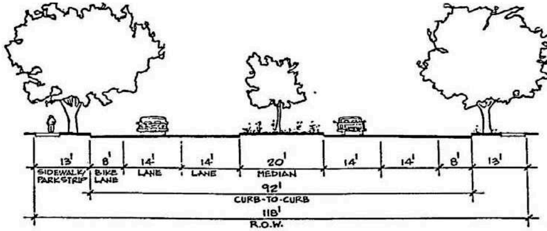
Figure 2-3C Divided Arterial (General Plan Drawing)
