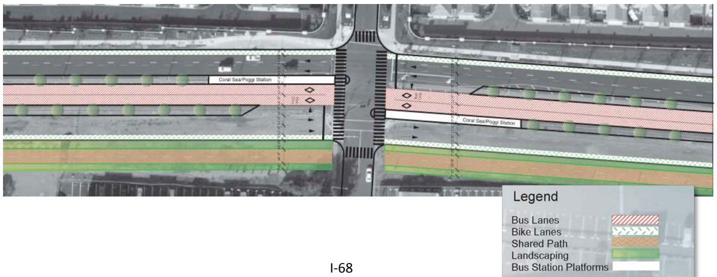
Figure 3-4 Transitway Design for Bus Rapid Transit (Concept)
