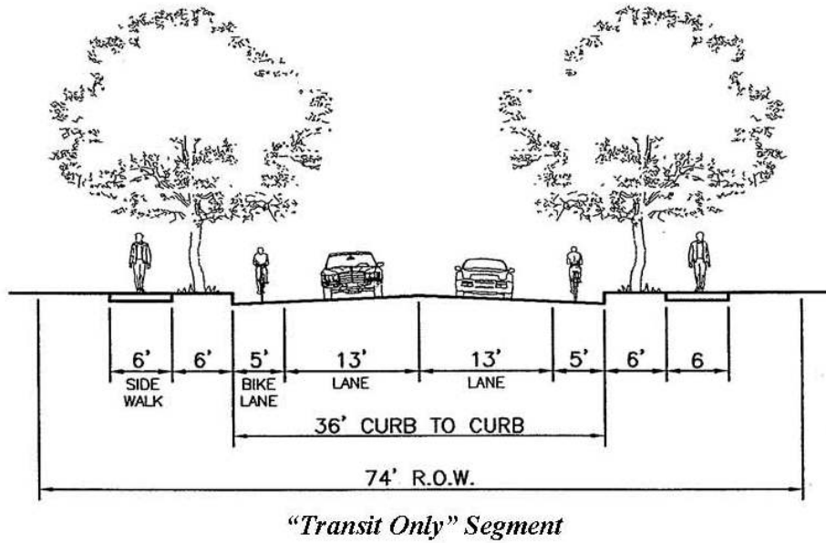
Figure 2-3E Transitway (General Plan Drawing)
