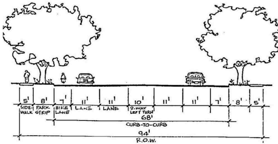
Figure 2-3D Minor Arterial (General Plan Drawing)
