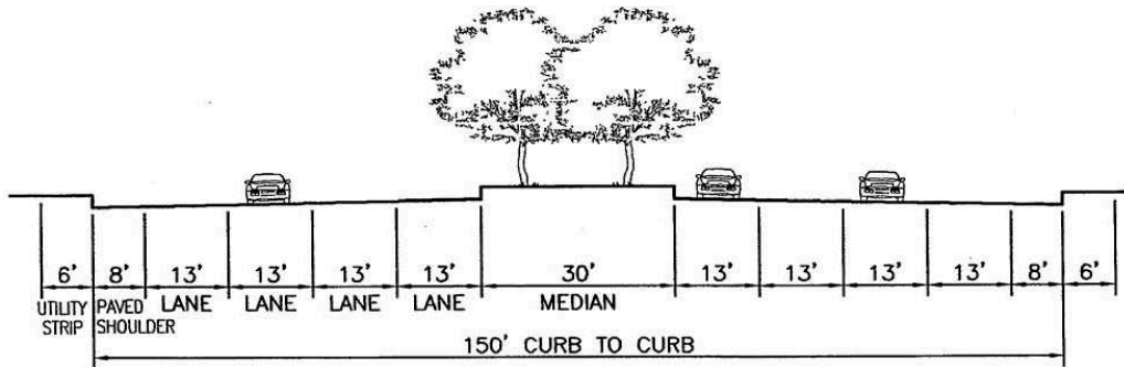
Figure 2-3B Major Arterial (General Plan Drawing)
