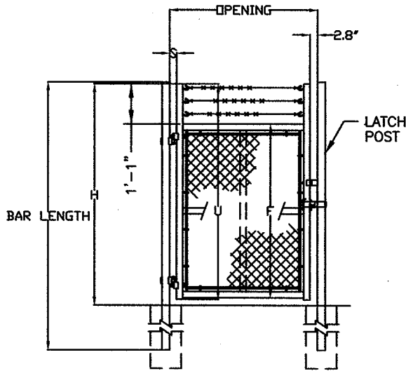
SINGLE GATE ELEVATION
