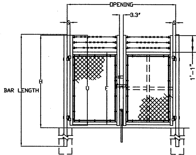
DOUBLE GATE ELEVATION
