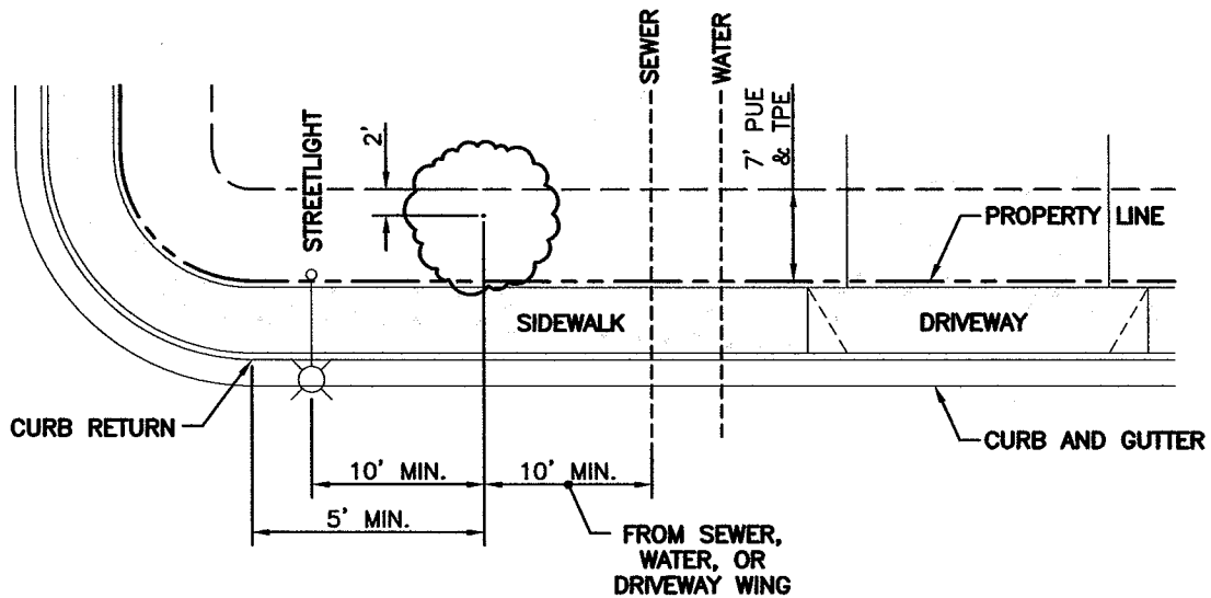
SIDEWALK ADJACENT TO CURB NO SCALE
