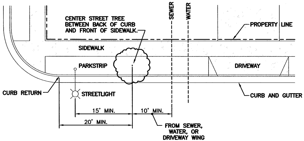
SIDEWALK AND PARKSTRIP NO SCALE
