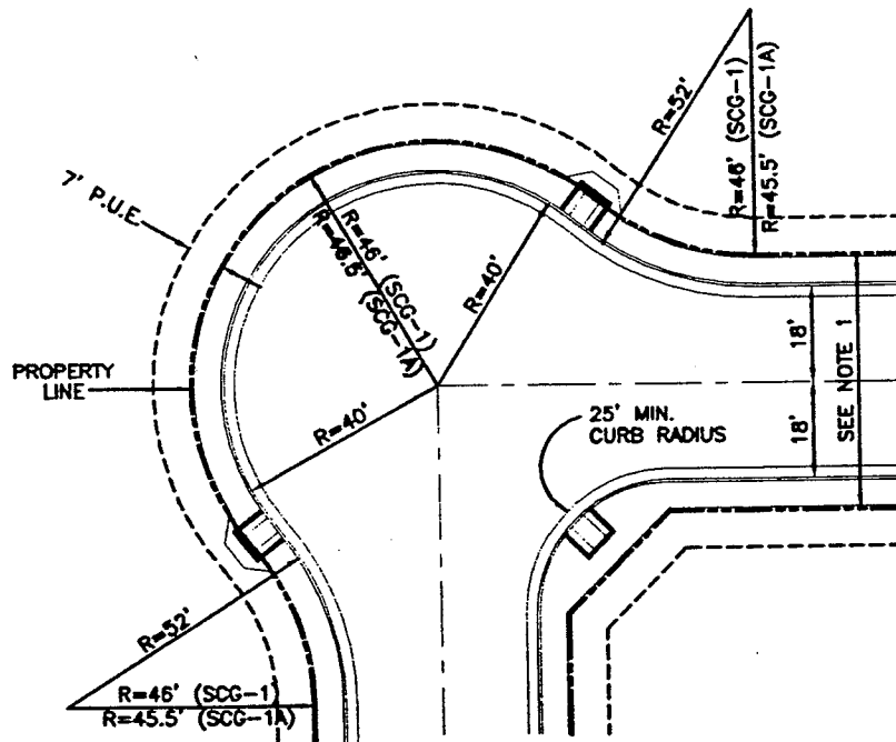
SIDEWALK ADJACENT TO CURB
